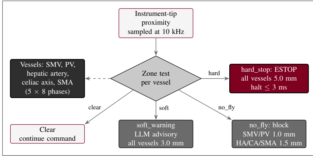
Figure 15. Five-vessel vascular safety-zone gate for Arm A. Three concentric proximity zones around each vessel drive response: a soft-warning zone raises an LLM advisory, a no-fly zone (superior mesenteric and portal veins; hepatic artery, celiac axis, and superior mesenteric artery) blocks the command, and a hard stop zone forces a cross-arm E-stop. The gate is sampled at 10 kHz across all eight phases of the operation.
