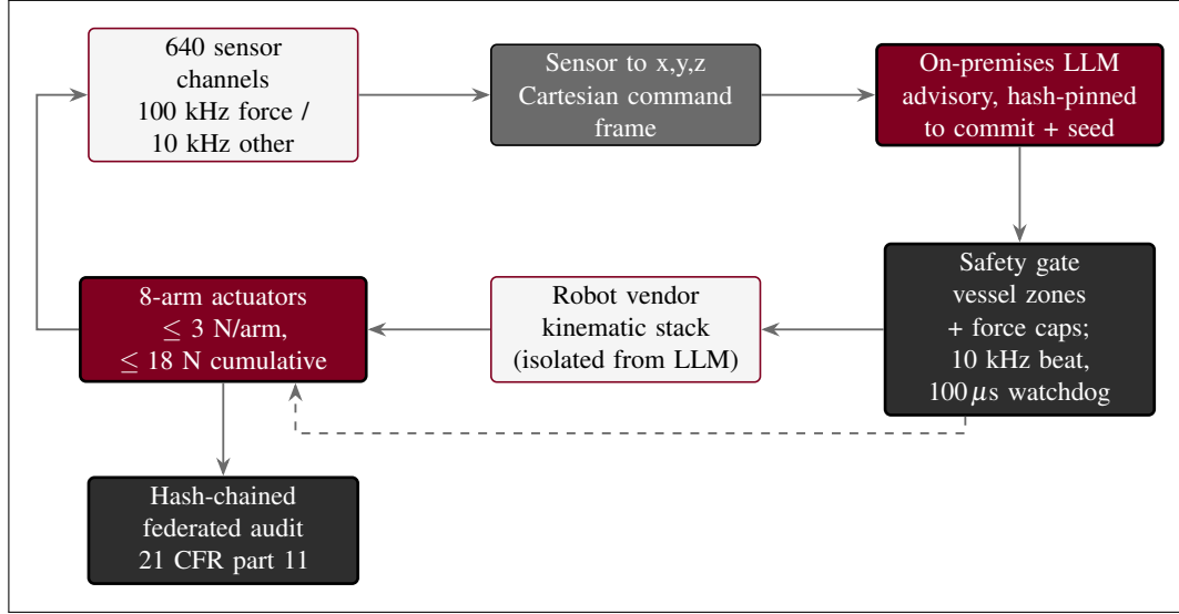
Figure 11. On-premises LLM advisory control loop. Sensor data is mapped to a Cartesian command frame; the LLM issues hash-pinned advisory commands from outside the vendor kinematic stack (second-opinion oracle isolation); and a safety gate enforces the vessel zones, the force caps, the 10 kHz heartbeat, and the 100 \mu s watchdog before any actuator moves. Actuator telemetry returns to the sensor stack, and every step is written to a hash-chained federated audit trail under 21 CFR part 11 [5].
